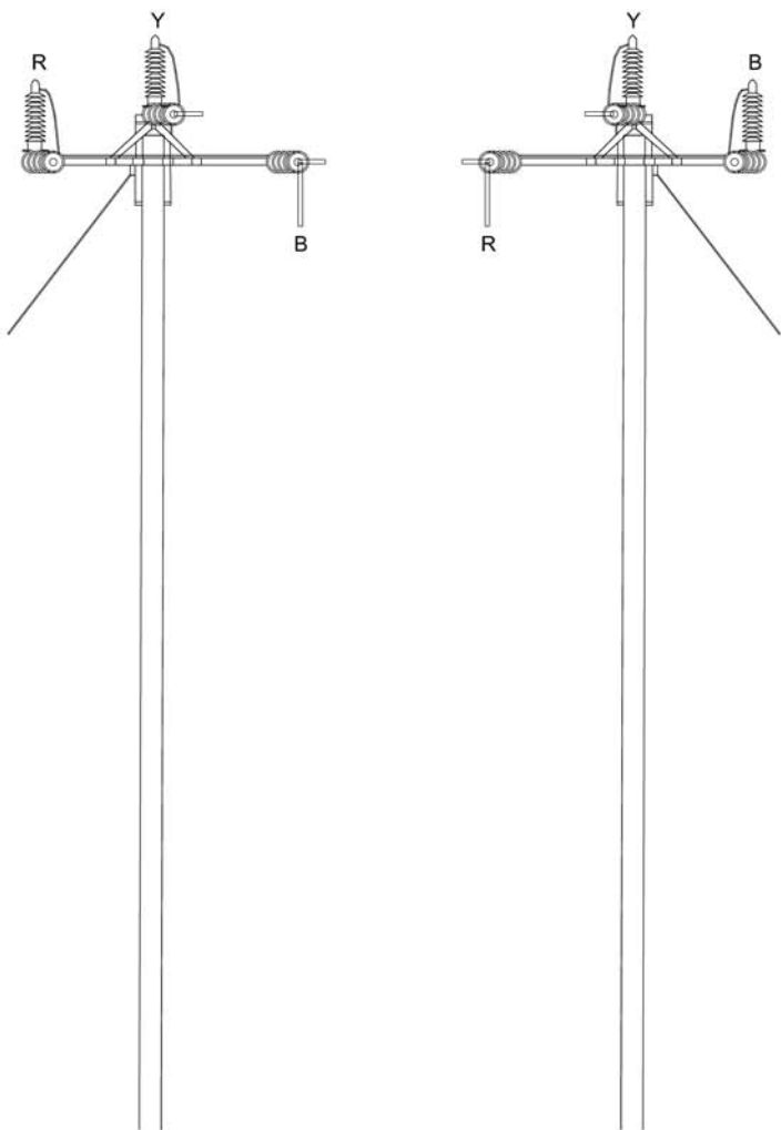
SINGLE POLE ARRANGEMENT
