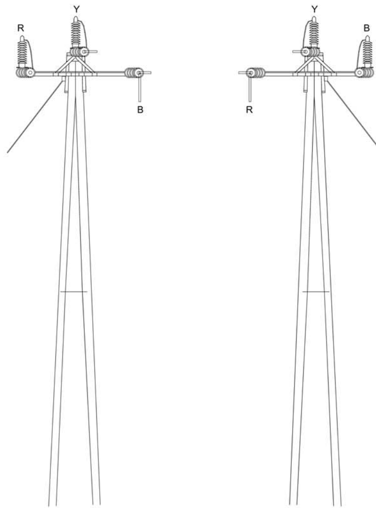
SECTION 'A' POLE ARRANGEMENT
